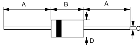
DO-201
